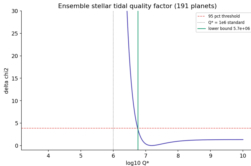
Figure 2. Joint constraint on the reduced stellar tidal quality factor Q' from the 191 planets entering the ensemble. The curve shows \Delta\chi^2 relative to the plateau as a function of \log Q' , evaluated on a 600-point
