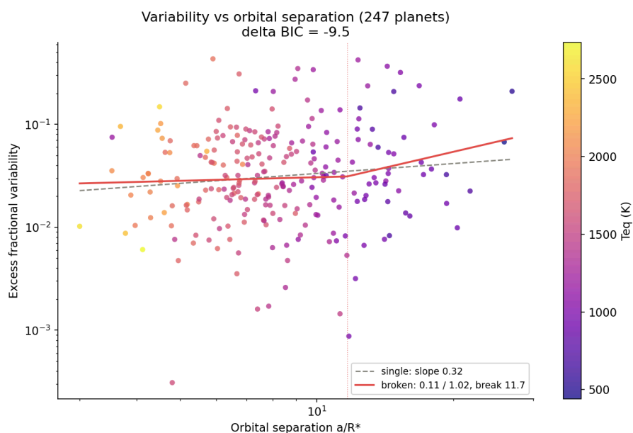
Figure 6. Excess fractional transit-depth variability against scaled orbital separation a/R^* for the 247 planets with positive excess, each coloured by equilibrium temperature. The dashed grey line is the best-fitting single power law, of slope 0.32 \pm 0.33 from 1000 bootstrap resamples, consistent with zero. The solid red line is the best-fitting continuous broken power law, disfavoured relative to the single power law by \Delta BIC = 9.5 . Neither the predicted rise with decreasing separation nor a break at the transition to the tidally dominated regime is detected.
