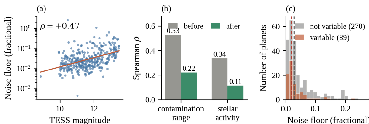
Figure 5. Validation of the injection–recovery noise floor. (a) Recovered noise floor against host-star TESS magnitude; the floor increases toward fainter stars ( \rho = +0.47 , p = 3 \times 10^{-21} ), the dependence expected of an instrumentally limited quantity. (b) Correlation of fractional variability with aperture contamination range and with stellar activity amplitude, before and after floor subtraction, falling from \rho = +0.53 to +0.22 and from \rho = +0.34 to +0.11 respectively. (c) Distributions of noise floor for the 89 planets classified variable and the 270 not so classified; variable planets have systematically lower floors (median 1.9 against 2.8 per cent, Mann–Whitney p = 0.004 ), the opposite of the expectation were the detected variability instrumental in origin.
