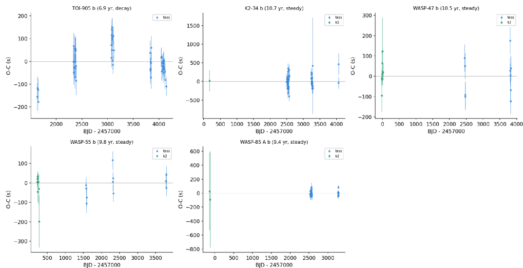
Figure 9. Observed-minus-calculated transit timing residuals, in seconds, for the anomalous system TOI-905 b and for the four planets with the longest baselines, plotted against barycentric Julian date. Residuals are computed against the refined linear ephemeris fitted in this work; error bars are the per-epoch timing uncertainties. TESS epochs are shown in blue and K2 epochs in green, the latter extending baselines to as much as 10.7 years. The clustering of TOI-905 b's 51 epochs into five temporally separated groups is the configuration that permits a spurious parabolic fit.
