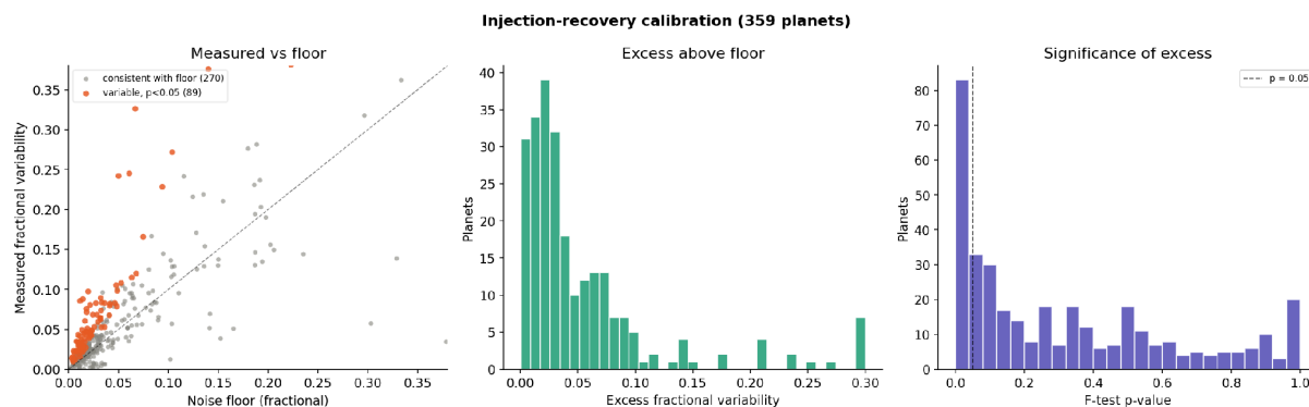
Figure 4. Injection–recovery calibration for the 359 planets with successful noise-floor measurements. Left: measured fractional transit-depth variability against each planet's own instrumental noise floor, with the dashed line marking equality; the 89 planets whose measured variance exceeds their floor at F-test significance p < 0.05 are shown in orange and the remaining 270 in grey. Centre: distribution of excess fractional variability after the floor is removed in quadrature. Right: distribution of F-test p -values, with the dashed line at p = 0.05 ; the concentration of values near zero against an otherwise approximately flat distribution indicates a detected population rather than noise alone.
