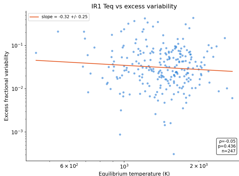
Figure 7. Excess fractional transit-depth variability against equilibrium temperature for the same 247 planets. The solid line is the best-fitting power law; the inset reports the Spearman rank correlation coefficient, its p -value and the sample size. No dependence on equilibrium temperature is detected ( \rho = -0.05 , p = 0.44 ), contrary to the prediction that variability should increase with stellar irradiation.
