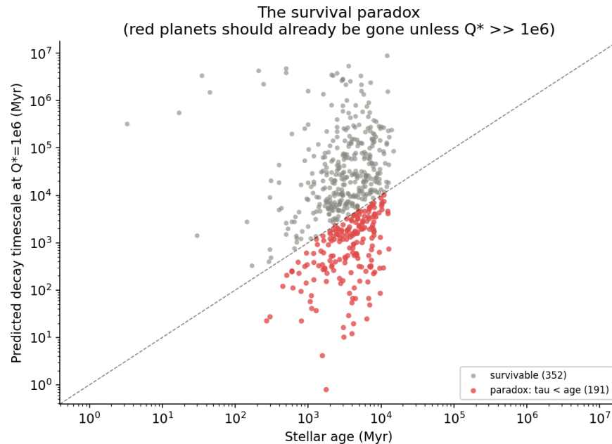
Figure 3. Predicted orbital decay timescale at Q' = 10^6 against host-star age, for the 543 planets with archive stellar ages. Points below the dashed one-to-one line have predicted decay timescales shorter than the age of their host star and so should not survive under that assumption; 191 systems (red) fall in this region against 352 (grey) that do not. Because the decay timescale scales linearly with Q' , the bound derived in this work rescales every point upward by a factor of approximately six, reducing the number of systems below the line to 70.
