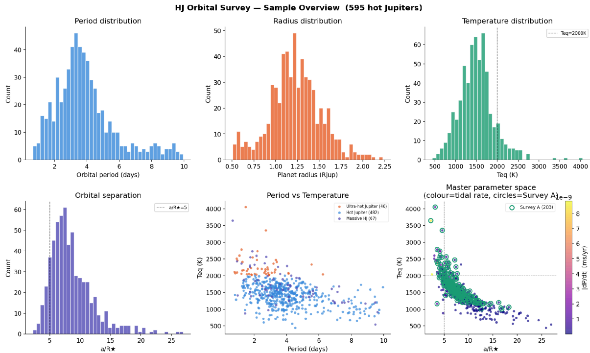
Figure 1. Distributions of the 595-planet hot Jupiter sample. Top row: orbital period, planetary radius in Jupiter radii, and equilibrium temperature, with the 2000 K ultra-hot boundary marked. Bottom row: scaled orbital separation a/R_* , with a/R_* = 5 marked; equilibrium temperature against orbital period, coloured by subtype (482 classical, 67 massive above 3 M_{Jup} , 46 ultra-hot above 2000 K); and equilibrium temperature against a/R_* , coloured by the tidal decay rate predicted at Q' = 10^6 , with the brighter subsample ( T_{mag} \leq 11 , T_{eq} \geq 1000 K) circled. The period distribution peaks at 3–4 days and the radius distribution near 1.2 R_{Jup} , reproducing the known hot Jupiter population.
