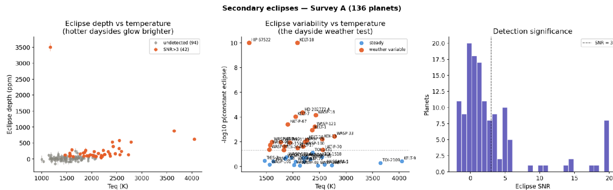
Figure 8. Secondary-eclipse measurements for the 136 planets of the brighter Survey A subsample. Left: measured eclipse depth in parts per million against equilibrium temperature; the 42 planets detected above \text{SNR} = 3 are shown in orange and the remainder in grey. The positive correlation among detections (Spearman \rho = +0.32 , p = 0.038 ) is the expected thermal-emission behaviour and validates the measurement. Centre: significance of the departure from constant eclipse depth against equilibrium temperature for the detected planets, with the dashed line at p = 0.05 and dayside-variable planets in orange; the variable fraction shows no systematic trend across 1175–2782 K. Right: distribution of eclipse detection significance, with the \text{SNR} = 3 threshold marked.
