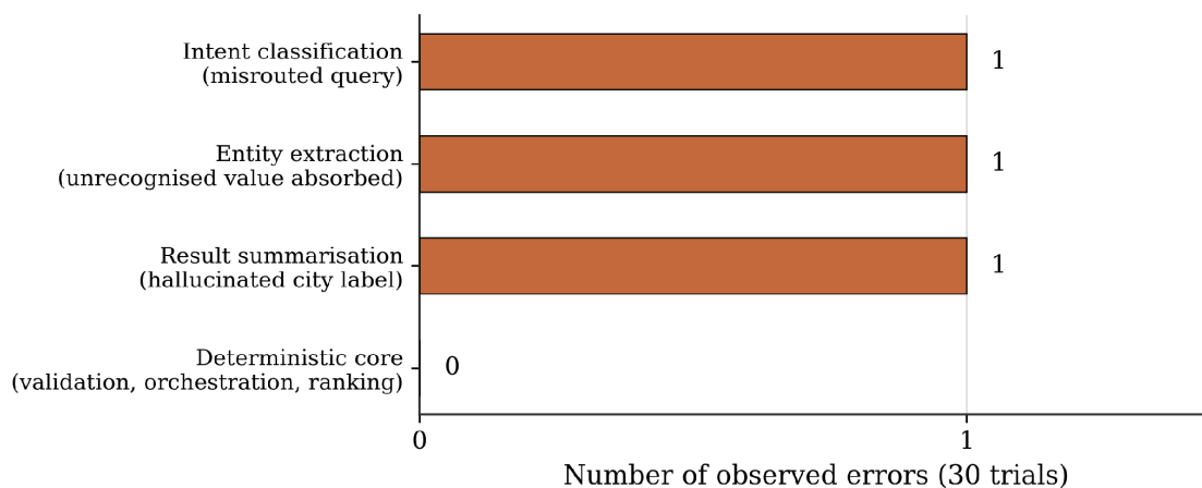
Figure 7. Distribution of observed errors by pipeline stage across 30 trials. All three instances arose at language-model stages; the deterministic core contributed none.
