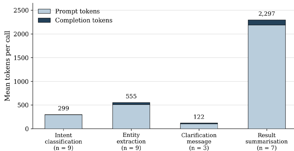
Figure 8. Mean prompt and completion tokens per GPT-4o call by reasoning function, measured over six instrumented conversations.
