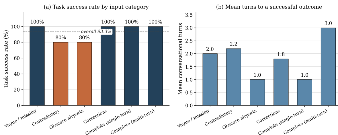
Figure 4. Task success rate (a) and mean conversational turns to a successful outcome (b), by input category. Categories containing a failure are shown in a contrasting color.
