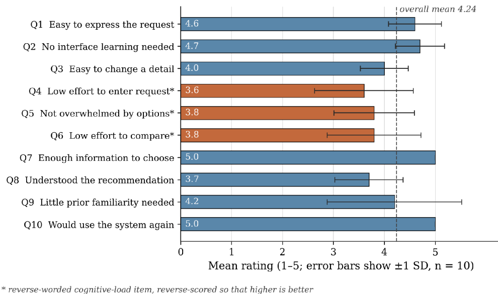
Figure 6. Mean usability rating by questionnaire item, with error bars showing one standard deviation ( n = 10 ). Reverse-worded cognitive-load items are shaded differently and are plotted reverse-scored.
