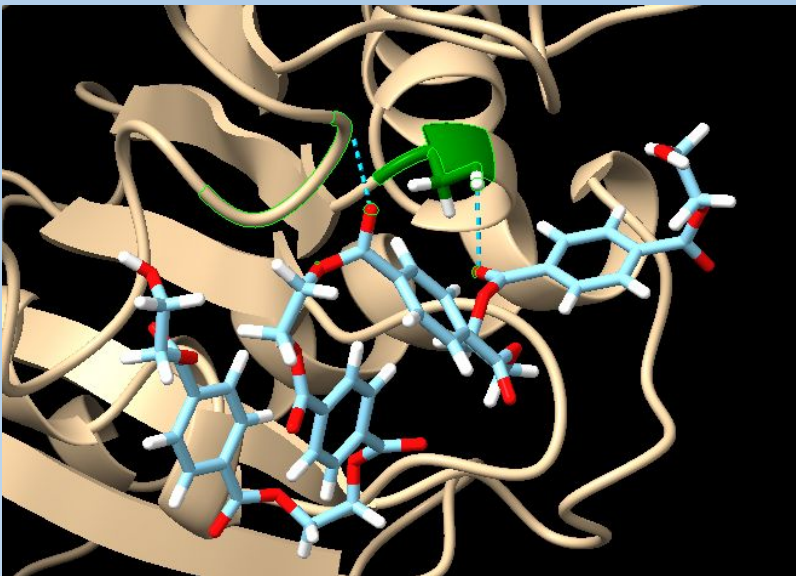
Figure 4: Example of the ChimeraX visualization-FASTPETase with 4-mer PET oligomer
