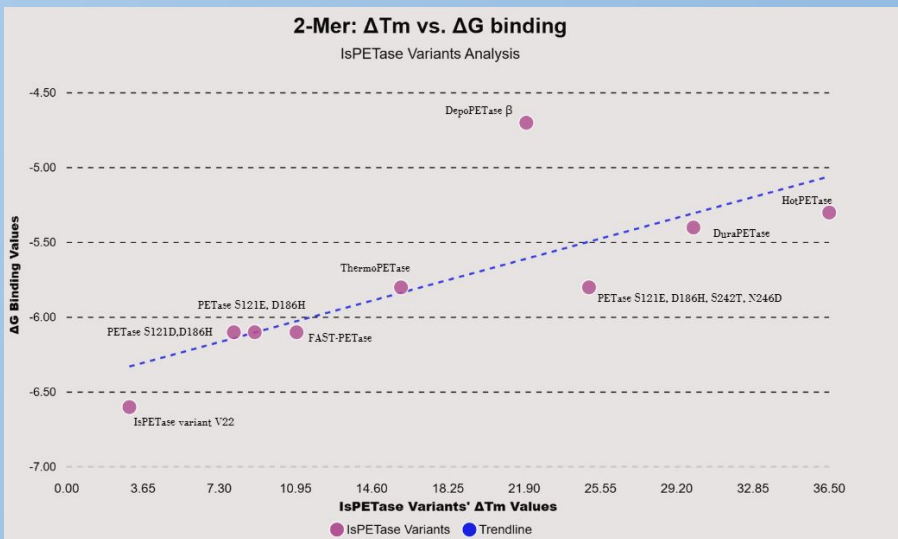
Figure 5: Scatter plot demonstrating a positive slope for the trendline between \Delta T_m and \Delta G binding: 2-mer
