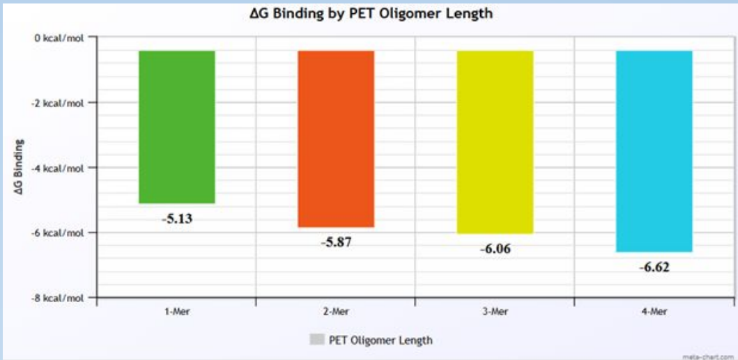
Figure 3: Bar graph demonstrating the average \Delta G binding for each PET oligomer length (1-4mer).
