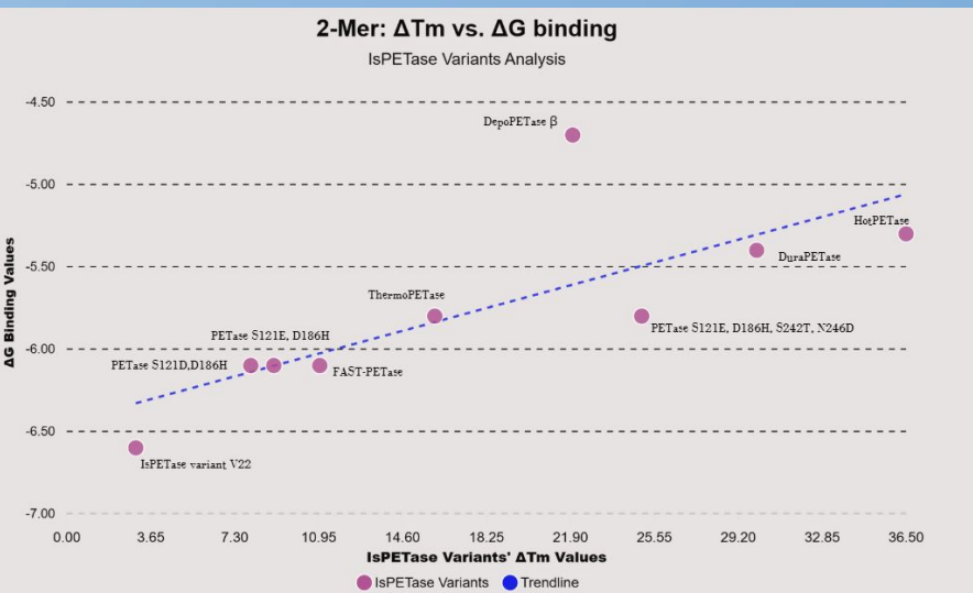
Figure 6: Scatter plot demonstrating a positive slope for the trendline between \Delta T_m and \Delta G binding: 2-mer
