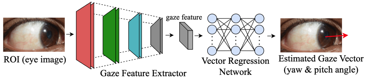
Figure 4. Network architecture of the proposed gaze estimation network
