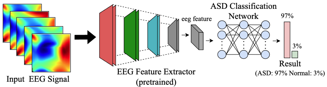
Figure 3. Network architecture of the proposed ASD classifier
