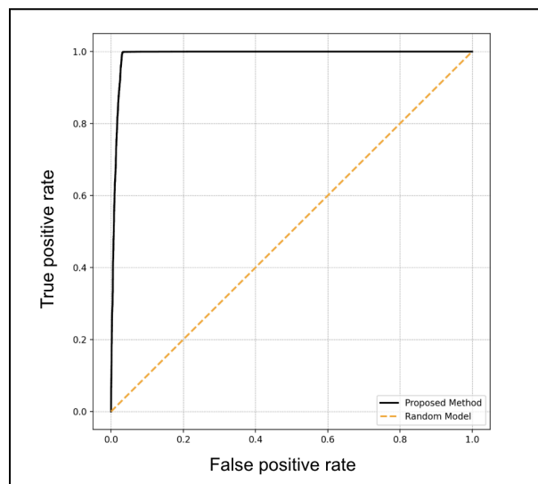
Figure 11. ROC curve of the proposed method
