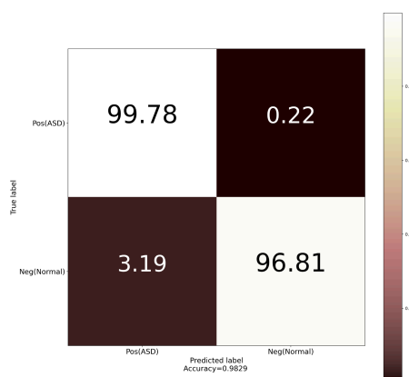
Figure 10. Confusion matrix for the proposed method.
