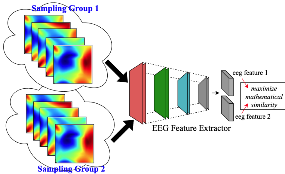
Figure 2. Network architecture of the proposed EEG representation learning
